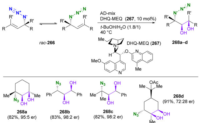
Scheme 51 Enantioselective dihydroxylation of the olefins under the Winstein rearrangement equilibrium.
