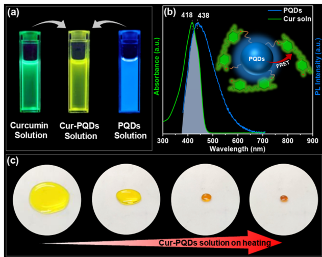
Fig. 2 (a) Digital images of Cur, Cur-PQDs, and PQDs solutions under UV light. (b) Spectral overlap of absorbance of Cur solution and emission band of PQDs (inset showing the FRET between PQDs and Cur molecules). (c) Photographs displaying the visual color change of Cur-PQDs solution on heating.
