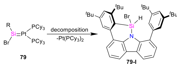
Scheme 27 Decomposition of 79 to 79-I .
