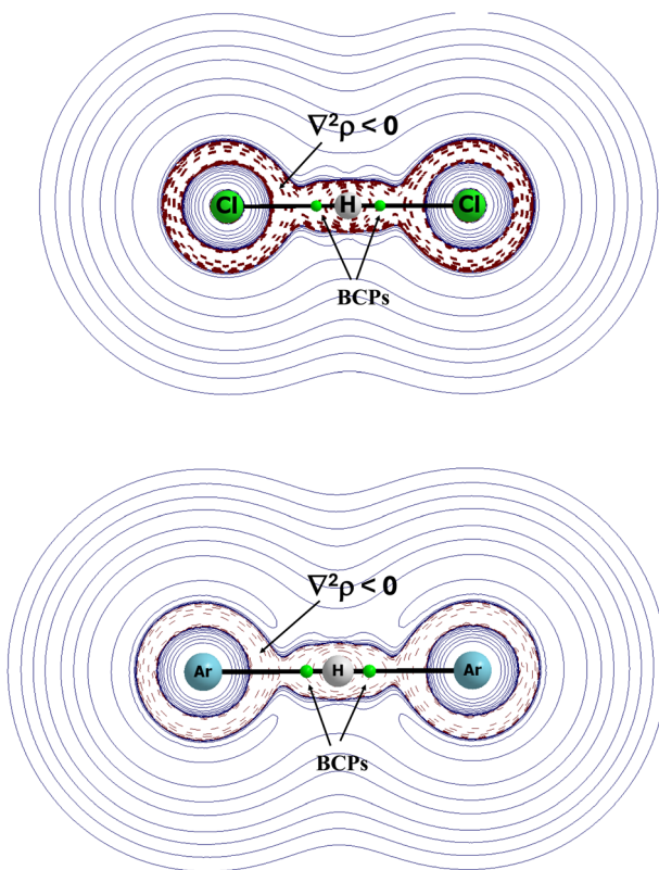
Fig. 8 The Laplacian of the electron density, \nabla^2\rho , for the (\text{ClHCl})^- anion (top) and for the (\text{ArHAr})^+ cation (bottom). The areas with the broken lines correspond to the negative values of \nabla^2\rho , small green circles correspond to bond critical points, and black lines between attractors correspond to bond paths.
