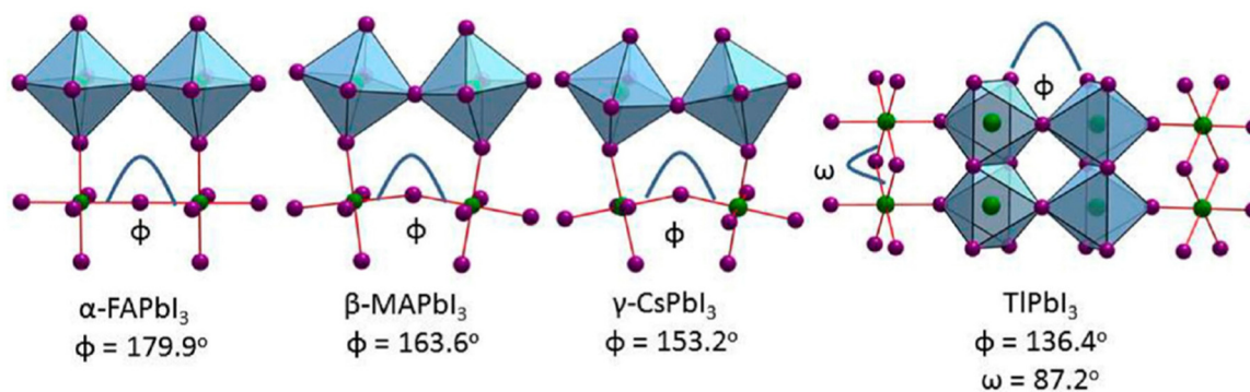
Fig. 1 Crystal structures of the APbI_3 series at room temperature for A = FA, MA, Cs, Tl, and NH_4 cations, highlighting the effect of the structural distortions and the connectivity of the [PbI_6]^{4-} octahedra. Adapted with permission from ref. 51.
