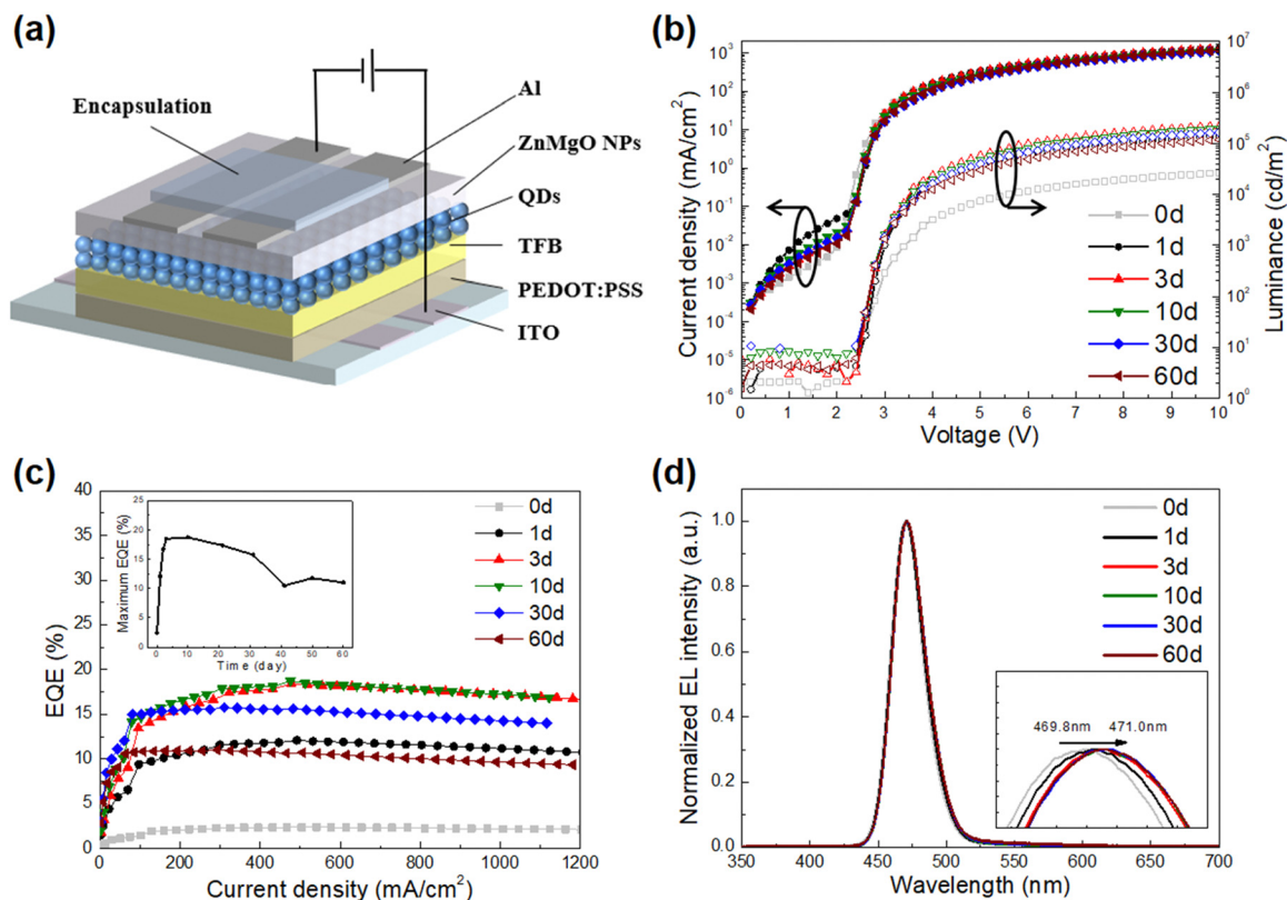
Fig. 1 (a) Device structure, (b) J - V - L , (c) EQE - J , inset is the EQE_{\max} changes over time. (d) EL spectra of blue QLEDs with encapsulation stored for different days in a nitrogen-filled glovebox.
