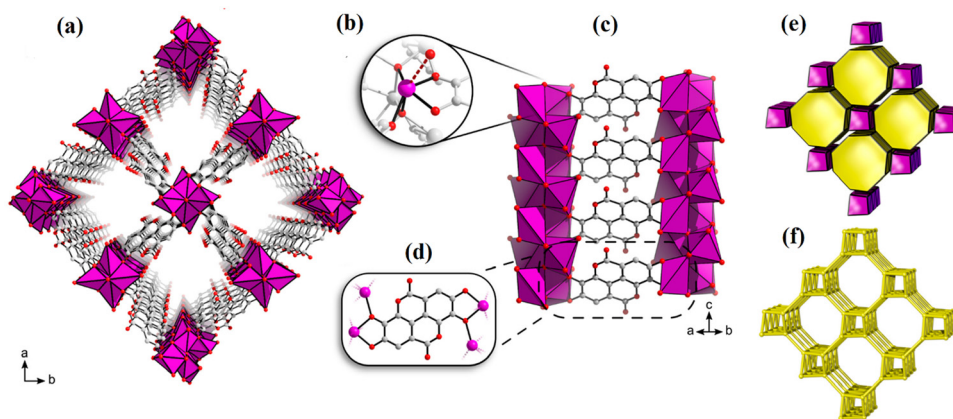
Fig. 5 Viewed along the c -axis, the SU-101 structure (a). The context for coordination surrounding \text{Bi}^{3+} (b). Chelation of ellagate toward bismuth oxo rods (c) and (d). The tiling of the svd net (e). The underlying svd net (f). Reproduced from ref. 99 with permission from the American Chemical Society.
