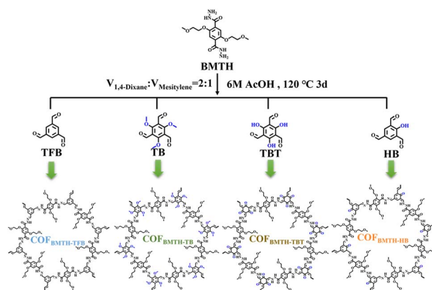
Scheme 1 Synthesis procedures and the structures of COF BMTT-TFB , COF BMTT-TB , COF BMTT-TBT and COF BMTT-HB .
