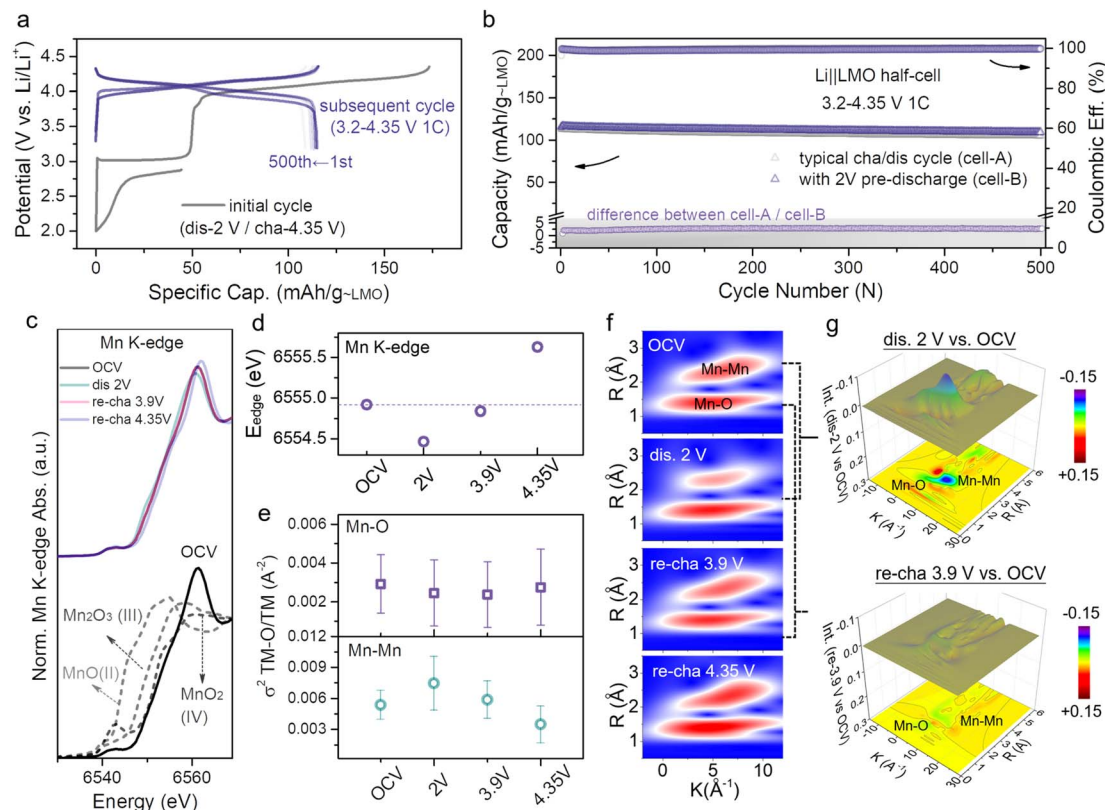
Fig. 2 (a) Voltage profiles of the Li||LMO half-cell that was initially discharged to 2 V and then cycled in the voltage range of 3.2–4.35 V (denoted as cell-B). (b) Cycling performances of cell-A (Fig. S9†) and cell-B, along with the difference of discharge capacity between cell-A and cell-B. (c) XANES spectra, and (d) edge positions at the Mn K-edge of the LMO electrodes at different voltage states. (e) Debye–Waller factor \sigma^2 , and (f) WT-EXAFS spectra of the Mn–O/Mn bond of the LMO at different states. (g) Color 3D WT-EXAFS spectra showing the differences between WT-EXAFS spectra of the Mn–O bond and Mn–Mn bond (first discharge to 2 V vs. OCV (top) and re-charge to 3.9 V vs. OCV (bottom)).
