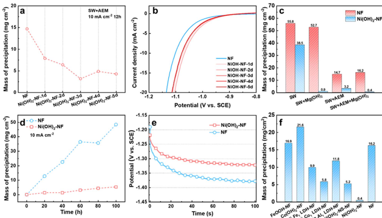
Fig. 3 (a) Mass of precipitation on the electrodes, and (b) the LSV curves of the electrodes under different deposition times. Mass of precipitation on the NF and \text{Ni}(\text{OH})_2\text{-NF} electrodes, (c) under different conditions, and (d) with different measure times. (e) Chronopotentiometry curves of NF and \text{Ni}(\text{OH})_2\text{-NF} electrodes with the electrolyte replaced every 20 h under a current density of 10 \text{ mA cm}^{-2} . (f) Mass of precipitation on the different kinds of hydroxide-decorated electrodes.
