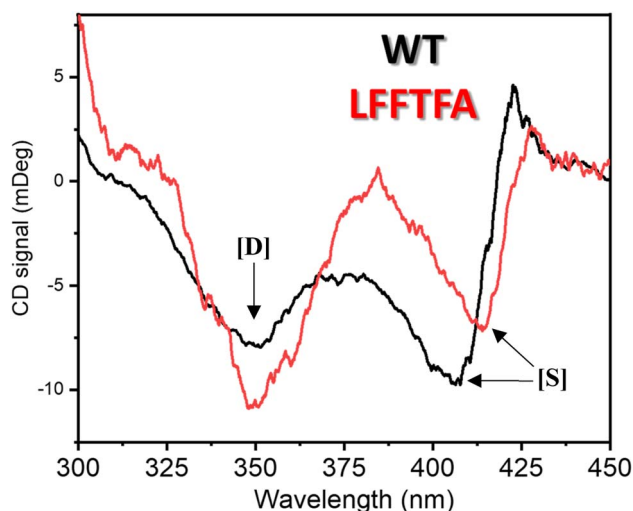
Fig. 7 CD spectrum of substrate free wild-type (black) and the LFFTF A mutant (red) of CYP175A1 in the 300–450 nm region showing the Soret and delta bands. [D] denotes the delta band and [S] denotes the Soret band.
