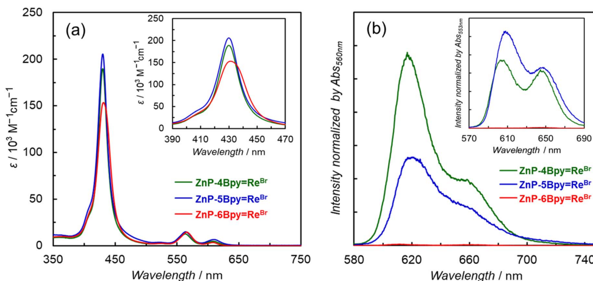
Fig. 4 (a) UV-vis absorption spectra of \text{ZnP-}n\text{Bpy=Re}^{\text{Br}} ( n = 4, 5 , and 6 ) in DMA. Inset shows magnification of the Soret bands. (b) Fluorescence spectra of \text{ZnP-}n\text{Bpy=Re}^{\text{Br}} ( n = 4, 5 , and 6 ) in Ar-saturated DMA ( \lambda_{\text{ex}} = 560 \text{ nm} ) at 298 \text{ K} . Inset shows spectra in Ar-saturated toluene ( \lambda_{\text{ex}} = 553 \text{ nm} ) at 298 \text{ K} . The fluorescence spectra were normalized with absorbance at the excitation wavelength.
