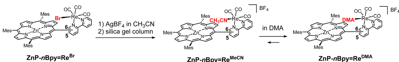
Scheme 2 Synthesis of \text{ZnP-}n\text{Bpy=Re}^{\text{MeCN}} and ligand substitution of acetonitrile to DMA.
