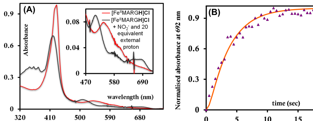
Fig. 7 (A) Absorption spectra of [\text{Fe}^{\text{II}}\text{MARGH}]\text{Cl} (red) upon simultaneous addition of 5 equivalents of [\text{NBu}_4]\text{NO}_2 and 20 equivalents of 2,6-xylydinium chloride (dark grey). (B) Kinetic trace followed at 692 nm regarding the formation of \text{Fe}^{\text{III}}\text{-Cl} species when nitrite and 20 equivalents of 2,6-xylydinium chloride are added to [\text{Fe}^{\text{II}}\text{MARGH}]\text{Cl} simultaneously.
