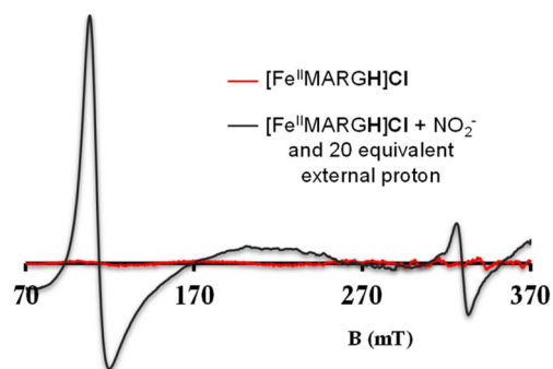
Fig. 8 X-band EPR spectra of [\text{Fe}^{\text{II}}\text{MARGH}]\text{Cl} (red) upon simultaneous addition of 5 equivalents of [\text{NBu}_4]\text{NO}_2 and 20 equivalents of 2,6-xylydinium chloride (dark grey).
