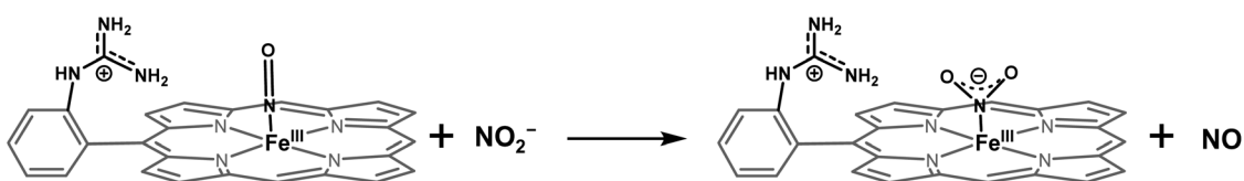
Scheme 3 Schematic representation of NO displacement from {FeNO} 6 species of [MARGH]Cl by the π anisotropic NO 2 - ligand.
