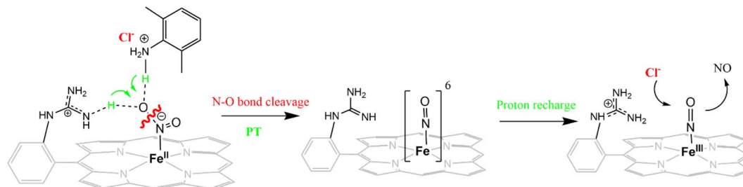
Scheme 2 Schematic representation of NO displacement from {FeNO} 6 species of [MARGH]Cl by Cl - ligand upon simultaneous addition of 20 equivalents of 2,6-xylylidinium chloride with [NBu 4 ]NO 2 to [Fe II MARGH]Cl complex.
