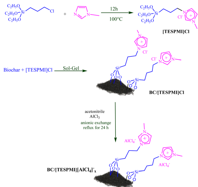
Scheme 1 General scheme for preparation of BC/[TESPMI] \text{AlCl}_4 catalyst.
