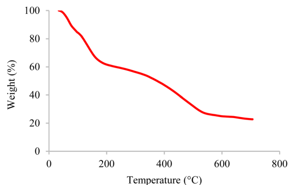
Fig. 2 The TGA curve of BC/[TESPMI] \text{AlCl}_4 catalyst.
