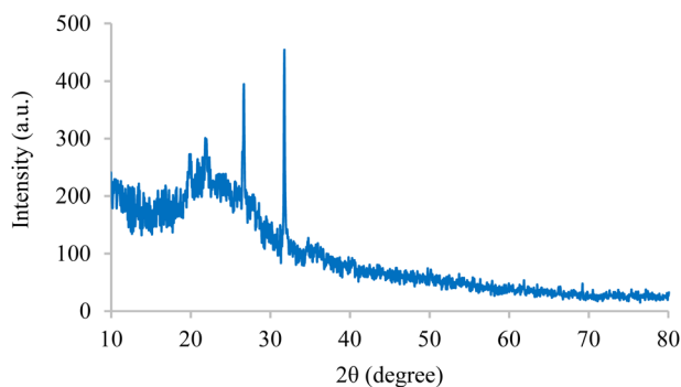
Fig. 1 The XRD pattern of BC/[TESPMI] \text{AlCl}_4 catalyst.
