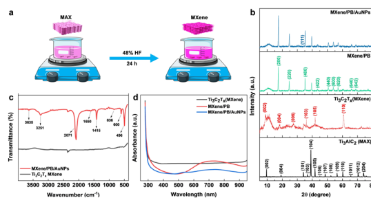
Fig. 1 (a) Schematic diagram of the synthesis of \text{Ti}_3\text{C}_2\text{T}_x MXene from \text{Ti}_3\text{AlC}_2 MAX phase by acid etching method. (b) XRD pattern of \text{Ti}_3\text{AlC}_2 MAX phase, \text{Ti}_3\text{C}_2\text{T}_x MXene, MXene/PB, and MXene/PB/AuNPs nanocomposite. (c) FT-IR spectra of MXene and MXene/PB/AuNPs, and (d) UV-vis spectrum of MXene, MXene/PB, and MXene/PB/AuNPs.
