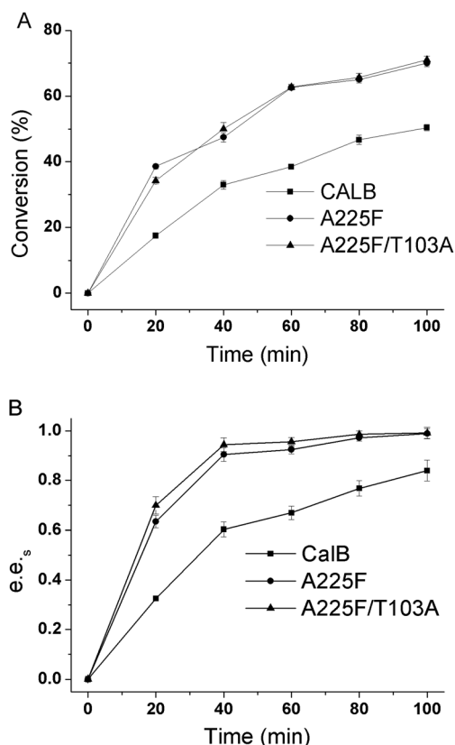
Fig. 6 Conversion time courses and e.e.s time courses of CALB and mutant catalysis of ( R , S )-1 (1,4-benzodioxane-2-carboxylic acid methyl ester). (A) Conversion time course of CALB and mutant catalysis of ( R , S )-1; (B) e.e.s time courses of CALB and mutant catalysis of ( R , S )-1.
