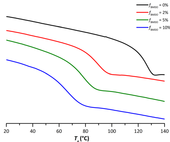
Fig. 6 Thermograms from DSC analyses performed on the dried extract of latexes of PMMA (E1MMA) and P(MMA-co-BMDO) with increasing amounts of BMDO: f_{\text{BMDO},0} = 2\% (E4BMDO), f_{\text{BMDO},0} = 5\% (E1BMDO), f_{\text{BMDO},0} = 10\% (E5BMDO) (Table 1).
