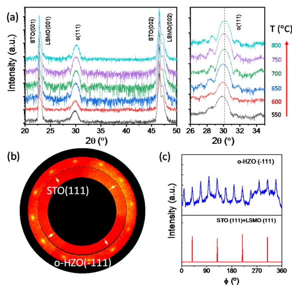
Fig. 1 (a) XRD \theta – 2\theta scans of HZO films deposited on STO(001) at the temperature indicated on the right. Scans are shifted vertically for clarity. The enlarged 2\theta region shown in the right panel was scanned with a longer acquisition time. The dashed vertical line marks the position of the peak in the T_s = 800 °C sample. (b) Pole figures and (c) \phi -scans around the o-HZO(–111) and STO(111) reflections of the T_s = 550 °C sample.
