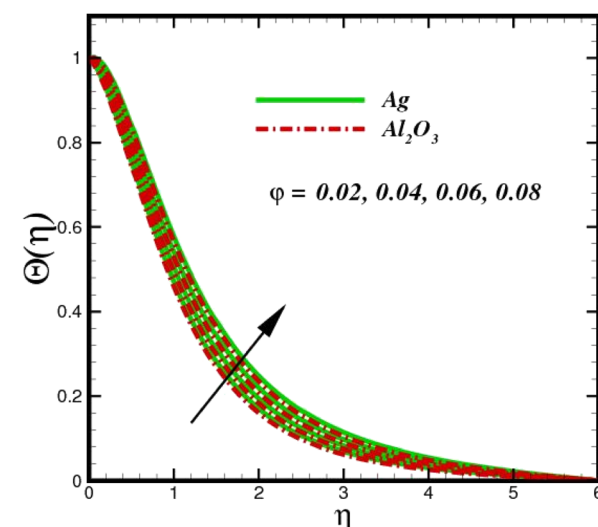
Fig. 9 Temperature sketch \Theta(\eta) with the upshot in \phi .
