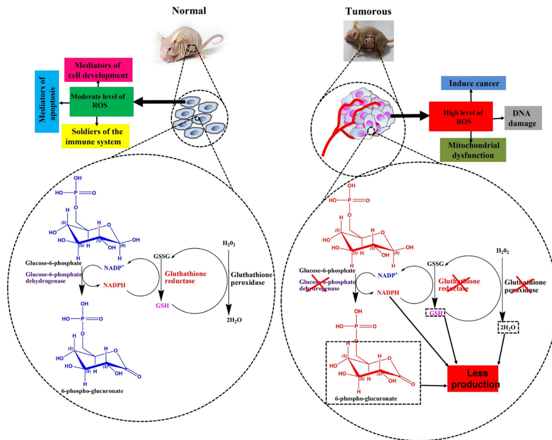
Fig. 13 Diagrammatic view of glucose-6-phosphate dehydrogenase reaction and the levels of glutathione (GSH), nicotinamide adenine dinucleotide phosphate (NADPH), and hydrogen peroxide ( \text{H}_2\text{O}_2 ) in normal and tumorous cells.
