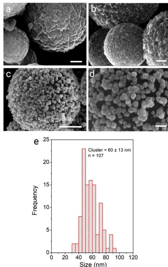
Fig. 3 SEM micrographs of precursor and composite systems prepared using approach 2: (a) CA-CμP , (b) CμP-AuNP(BH) and (c and d) roughened composites CμP-AuNP-2 . Scale bars show (a and b) 100 nm; and (d) 50 nm.
