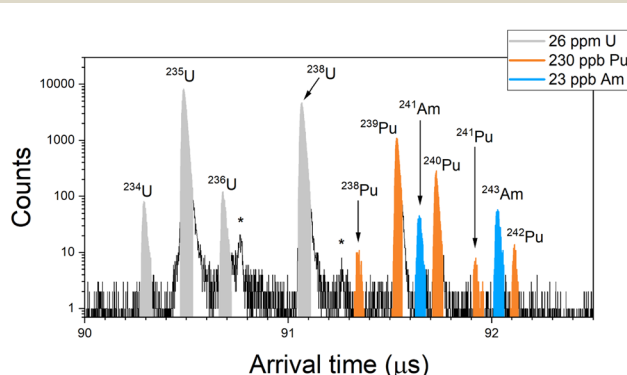
Fig. 1 RIMS spectrum of sample BCR-2B in the simultaneous analysis mode. Colored peaks correspond to U, Pu, and Am. Peaks marked with asterisks are due to non-resonant ion production as explained in the text.
