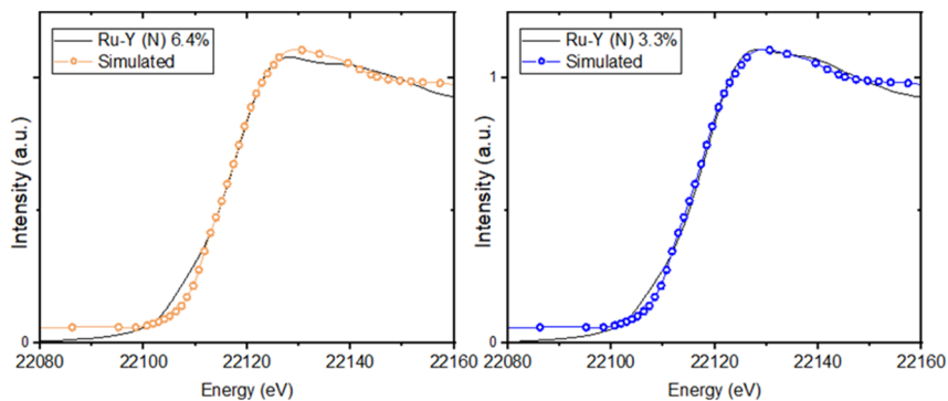
Fig. 11 Simulated XANES spectra at the Ru-K edge of Ru 6 N 6 cluster, compared with experimental Ru-Y (N) 6.4% and Ru-Y (N) 3.3% XANES (also see ESI†).
