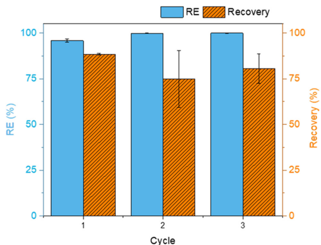
Fig. 8 Adsorption removal efficiency (blue) and desorption recovery (orange) for three cycles of regeneration of FLG@TA@RSN adsorbent. For adsorption, a BaP aqueous solution of 10 \mu\text{g L}^{-1} was prepared with 1% ethanol. An adsorption experiment was performed using 5 mg L -1 CN adsorbent for 15 min. For desorption, 2 mL of acetonitrile was used and desorption was performed for 10 min in an ultrasound bath. The vertical error bars correspond to the standard deviation determined from the two replicates. The removal efficiencies of the adsorption experiments were corrected for glassware adsorption based on blank experiments performed (see Fig. S7†).
