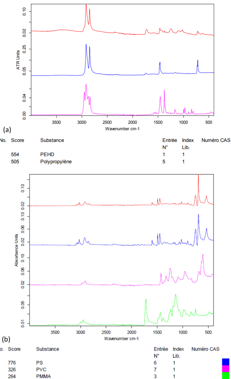
Fig. 1 a) Fourier transform infrared (FT-IR) spectrum of the environmental nanoplastic suspension NP-L (in red), best matching the tabulated spectra of PE and PP in the database (PE and PP); b) FT-IR spectrum of the NP-PS suspension (in red) compared to those of other standard vinylic polymers in the database (PS, polyvinyl chloride (PVC) and poly(methyl methacrylate) (PMMA)).
