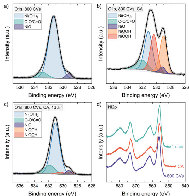
Fig. 4 XPS spectra of the fitted O1s and Ni2p regions of a 6 nm NiO thin film after an activation treatment of 800 CVs. a) with 800 CVs, NiO was almost completely transformed to Ni(OH)₂. b) after CA at 1.55 V vs. RHE, NiOOH is detected. c) Keeping the portion of the NiO peak constant in the fitting of the O1s region, little NiOOH is needed to fit the spectrum after storing the sample for one day in atmospheric conditions. d) Ni2p lines after 800 CVs, CA, and storage in air.
