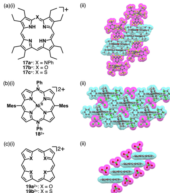
Fig. 10 (a) (i) Heteroatom-containing porphyrins 17a-c + and (ii) single-crystal X-ray structure of 17a + - \text{BAR}^{\text{F}-} , (b) (i) tetraaryl-5,15-diazaporphyrin Ni II complex 18 2+ and (ii) single-crystal X-ray structure of 18 2+ - 2\text{SbCl}_6^- and (c) (i) core-modified porphyrins 19a,b 2+ and (ii) single-crystal X-ray structure of 19a 2+ - 2\text{ClO}_4^- . The crystal structures are redrawn from cif files: 2033992, 1437728 and 1166405. Atom colour codes in (b) (c) (ii) and the following figures: green, blue-green and purple in the ball-and-stick models refer to chlorine, nickel and antimony, respectively.
