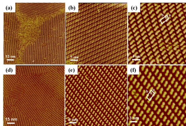
Fig. 7 Large-scale (a), medium range (b) and high-resolution (c) STM images of the self-assembly structure of \text{Tp}^6\text{Tt}_2\text{Tp}^6 on the 1-phenyloctane/HOPG interface (imaging parameters: (a): I_{\text{set}} = 299.1 pA, V_{\text{bias}} = 699.8 mV; (b): I_{\text{set}} = 247.2 pA, V_{\text{bias}} = 847.2 mV; and (c): I_{\text{set}} = 299.1 pA, V_{\text{bias}} = 699.8 mV); large-scale (d), medium range (e) and high-resolution (f) STM images of the self-assembly structure of \text{Tp}^8\text{Th}_2\text{Tp}^8 on the 1-phenyloctane/HOPG interface (imaging parameters: (d): I_{\text{set}} = 271.6 pA, V_{\text{bias}} = 770.0 mV; (e): I_{\text{set}} = 271.6 pA, V_{\text{bias}} = 770.0 mV; and (f): I_{\text{set}} = 271.6 pA, V_{\text{bias}} = 770.0 mV).
