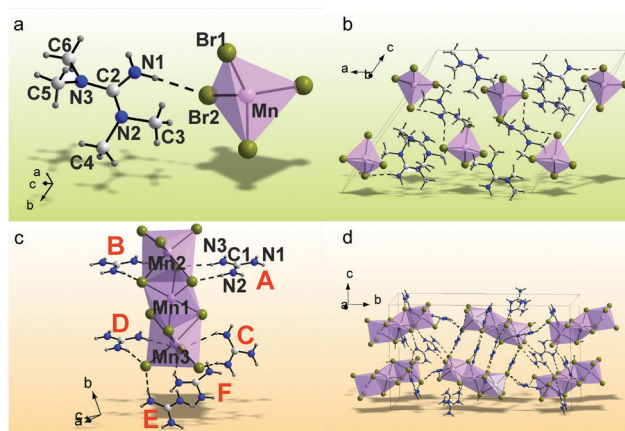
Fig. 1 Crystal asymmetric structure units of (\text{C}_5\text{H}_{14}\text{N}_3)_2\text{MnBr}_4 (a) and (\text{CH}_6\text{N}_3)_2\text{MnBr}_4 (c). The atoms in the asymmetric part of the unit cell of (\text{C}_5\text{H}_{14}\text{N}_3)_2\text{MnBr}_4 (b) and (\text{CH}_6\text{N}_3)_2\text{MnBr}_4 (d) are labeled, the hydrogen bonds in which are presented as dashed lines. The independent [\text{CH}_6\text{N}_3]^{2+} cations in the Figure (c) are marked by bold labels A–E.
