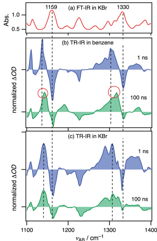
Fig. 6 (a) FT-IR spectrum of 2Cz2SB in KBr. TR-IR spectra of 2Cz2SB in (b) \text{N}_2 -saturated benzene and (c) KBr. TR-IR spectra at 1 and 100 \text{ ns} after photoexcitation are displayed as blue and green, respectively. Red circles indicate shift of frequencies.
