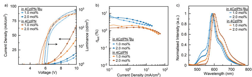
Fig. 4 (a) Comparison of current density–voltage–luminance ( J-V-L ) characteristics, (b) comparison of EQEs versus current densities, and (c) comparison of EL at EQE_{max} for OLED with binary blend EML.
