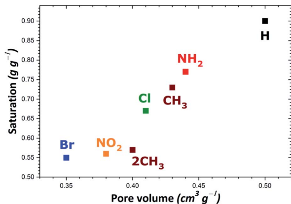
Fig. 1 \text{I}_2 adsorption capacity of the UiO-66 series with different functional groups based on its respective pore volume. Reproduced/adapted from ref. 36 with permission. 36
