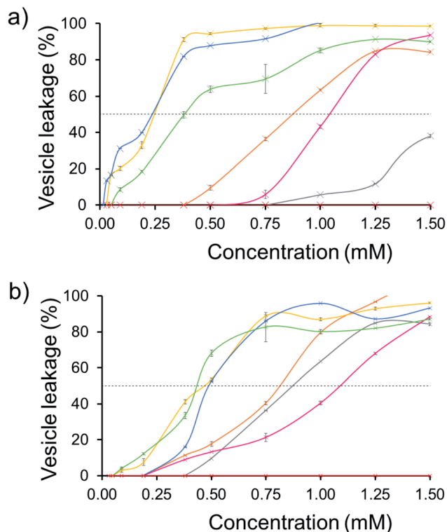
Fig. 6 The average ( n = 3 ) percentage lysis (%) of vesicles (30 \mu\text{M} ) composed of five different lipid compositions (Table 2), with an internal calcein concentration of 70 mM at 298 K. The % (a) PC and (b) PG vesicle lysis was calculated through observation of increasing fluorescence emission ( \lambda_{\text{em}} = 515 nm), following addition of SSA 5 (grey), SSA 6 (orange), SSA 8 (pink), SSA 9 (yellow), SSA 10 (blue), SSA 11 (green) and control solution 5% EtOH (red) after 15 min. Error = standard error. Black dotted line = 50% vesicle lysis.
