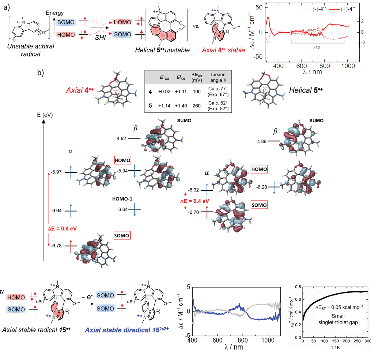
Fig. 13 (a) Axially and helically chiral SHI cationic bicarbazole monoradicals 4^{2+} and 5^{2+} , and orbital comparison with their common non-SHI cationic carbazole radical precursor, with the near IR circular dichroism of (+) and (–)- 4^{2+} (counter anions are omitted for clarity); (b) calculated orbital energies (in eV) and isosurfaces ( \pm 0.030 ) of frontier molecular orbitals computed for monoradicals 4^{2+} (left) and 5^{2+} (right). The HOMO–SOMO energy differences are averaged over the highest occupied spin orbital energies. Oxidation potentials and separation of the two first oxidation potentials in V vs. SCE, theoretical (calc.) and experimental (exp.) dihedral angles between the carbazole fragments; (c) schematic illustration of the electronic configuration of diradical 15^{2\cdot 2+} obtained upon oxidation of SHI radical 15^{2+} , near IR circular dichroism of (+) and (–)- 15^{2\cdot 2+} in acetonitrile at 298 K, and its magnetic susceptibility ( \chi_{\text{M}}T vs. T ). Figures adapted with permission from ref. 74. Copyright 2020 American Chemical Society.
