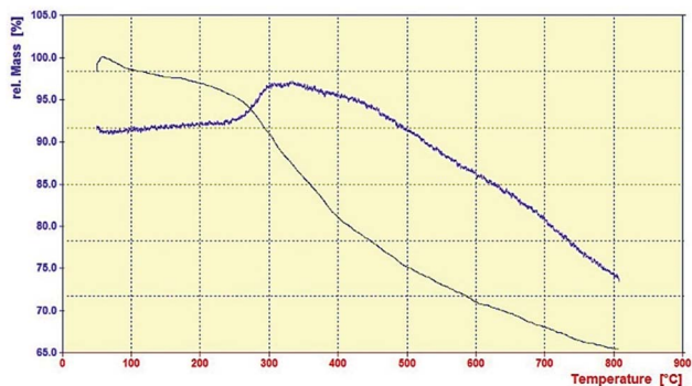
Fig. 8 TGA and DTA curves for PMAMOSa ( 1 ).
