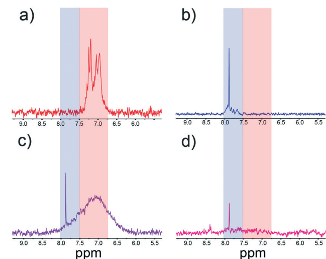
Fig. 9 1 H NMR spectra of (a) isolated raPTAK solution, (b) isolated PFPI solution, (c) PFPI/raPTAK complex solution, and (d) PFPI/raPTAK/liposome complex solution. The blue and red boxes largely correspond to PFPI and raPTAK aromatic resonance regions, respectively.
