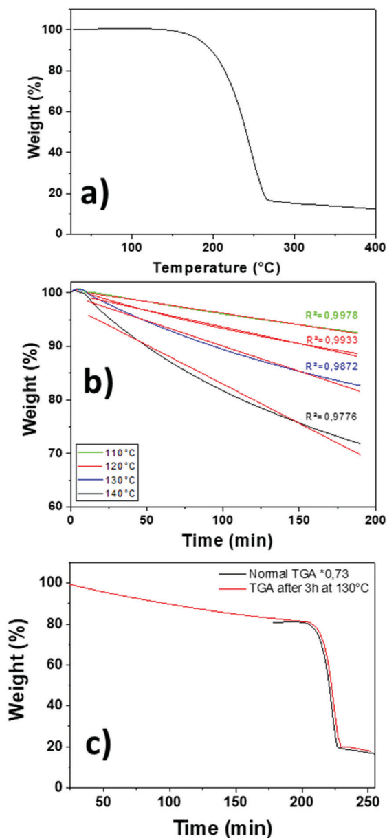
Fig. 1 (a) TGA of the precursor mixture ( \text{Bi}(\text{phenyl})_3 , \text{Fe}(\text{tmhd})_3 , and \text{Dy}(\text{hfa})_3 , diglyme). (b) Isothermal of the precursor mixture at various temperatures. (c) Comparison of the TGA curves of the precursor mixture and after 3 h isothermal at 130 °C.
