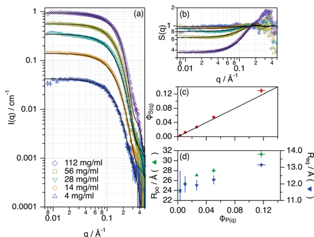
Fig. 2 (a) SANS data, (b) effective structure factor ( S(q) ) and best models for different concentrations of Lyz in ChCl : Glyc. The legend of the graph is presented in (a). (c) and (d) present the main results from the data analysis (effective structure factor volume fraction – \phi_{S(q)} , polar radius – r_{po} , and equatorial radius – r_{eq} ) as a function of the protein volume fraction – \phi_{P(q)} . Where not seen, the error bars are within the markers.
