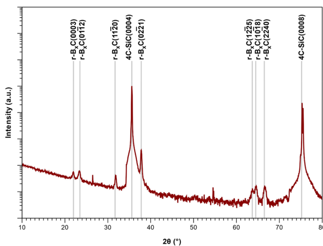
Fig. 6 2\theta/\omega diffractogram of a polycrystalline \text{B}_x\text{C} deposited at 1400 °C close to the inlet of the susceptor, corresponding to a residence time of 0.06 s. The sharp low-intensity non-indexed peaks come from the substrate.
