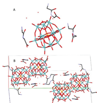
Fig. 3 The molecular (A) and crystal (B) structure of compound (HGlGly) 3 [PMo 12 O 40 ]·3H 2 O (3).
