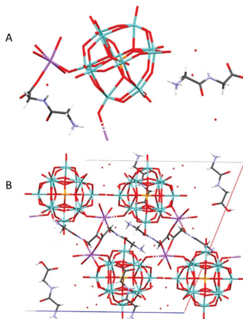
Fig. 5 The molecular (A) and crystal (B) structure of Na(HGlGly) 2 [PMo 12 O 40 ]·8H 2 O (5).
