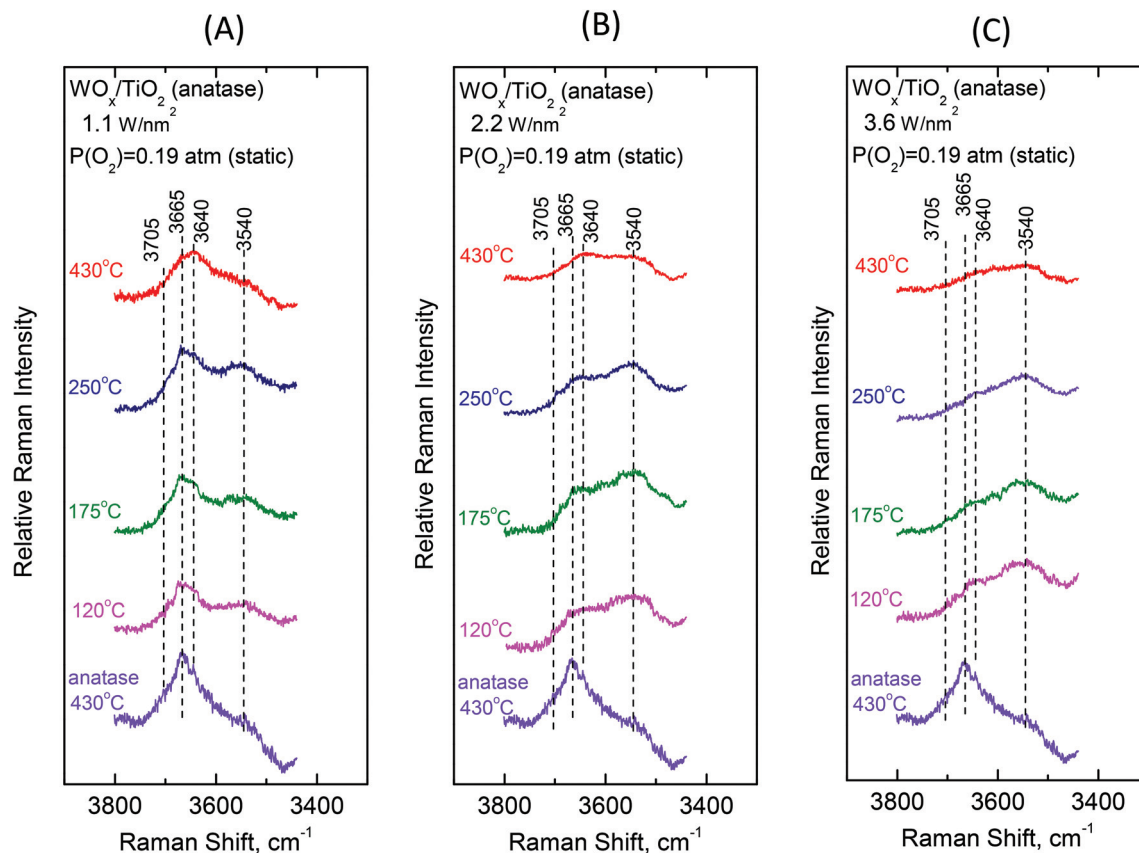
Fig. 11 \text{WO}_x/\text{TiO}_2(\text{anatase}) with surface density of (A) 1.1 \text{W}/\text{nm}^2 ; (B) 2.2 \text{W}/\text{nm}^2 ; and (C) 3.6 \text{W}/\text{nm}^2 . Sequential Raman spectra at static equilibrium under p_{\text{O}_2} = 0.19 atm at temperatures as indicated by each spectrum. Each panel includes the Raman spectrum of pure \text{TiO}_2(\text{anatase}) at 430 °C as reference. Spectral parameters: \lambda_0 = 532.0 nm; laser power, w = 20 mW; resolution, 2 \text{cm}^{-1} .
