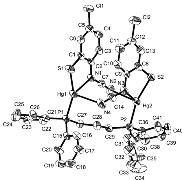
Fig. 5 Molecular structure of [\text{Hg}\{\text{SC}_6\text{H}_3\text{XN}(\text{C}\equiv\text{N})\}_2(\mu\text{-dppb})]_n ( 8c ). Thermal ellipsoids at the 50% level and hydrogen atoms are omitted for clarity. Selected bond lengths (Å) and bond angles ( ^\circ ): Hg1–N1 2.367(6), Hg1–N4 2.835(6), Hg2–N2 2.723(6), Hg2–N3 2.249(8), Hg1–S1 2.372(2), Hg2–S2 2.372(2), Hg1–P1 2.395(2), Hg2–P2 2.385(2), Hg1...Hg2 5.481(2), N1–C7 1.312(11), N2–C7 1.149(11), N3–C14 1.280(12), N4–C14 1.173(12); N1–Hg1–S1 81.06(18)^\circ , N1–Hg1–P1 114.72(18)^\circ , S1–Hg1–P1 157.36(8)^\circ , N3–Hg2–S2 81.6(2)^\circ , N3–Hg2–P2 122.5(2)^\circ , S2–Hg2–P2 155.74(8)^\circ .
