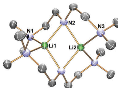
Fig. 3 X-ray crystal structure of [Li(μ-κ 2 -N,N'-N(CH 2 CH 2 NMe 2 ) 2 ) 2 ( 2 ) at −123 °C with 50% probability ellipsoids. Hydrogen atoms are omitted for clarity. The selected bond distances (Å) and angles (°) are: Li1–N1 2.0903(18); Li1–N2 2.0286(19); Li2–N2 2.0192(18); Li2–N3 2.0864(17); Li1...Li2 2.376(4); Li1–N2–Li2 71.89(9).
