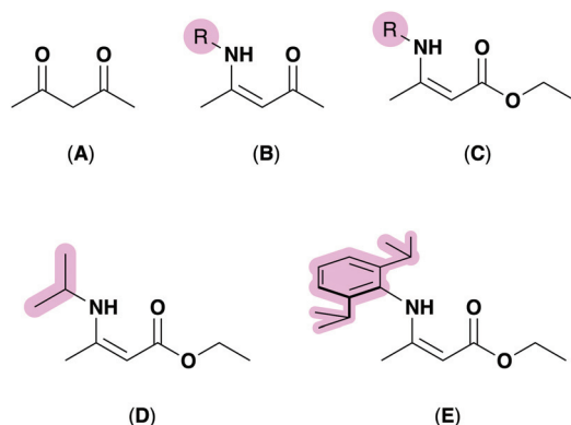
Fig. 1 Top: previously reported ligand systems for oxide formation include \beta -diketones (A), \beta -diketoinimes (B) and aminoenoates (C). Bottom: the aminoenoate pro-ligands employed in this work with i -Pr (D) and -Dip (2,6-diisopropylphenyl) (E) at the N-position. R-groups that can be tuned to vary precursor geometry, highlighted in pink.
