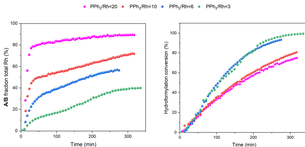
Fig. 5 Amount of A/B detected by quantitative ^1\text{H} FlowNMR spectroscopy during hydroformylation of 1-hexene under 12 bar of \text{CO}/\text{H}_2 (1 : 1) at 50^\circ\text{C} catalysed by [\text{Rh}(\text{acac})(\text{CO})_2] = 2.5 \text{ mM} and [\text{PPh}_3] = 7.5, 15, 25 and 50 \text{ mM} in 22.4 \text{ mL} of non-deuterated toluene versus conversion over time.
