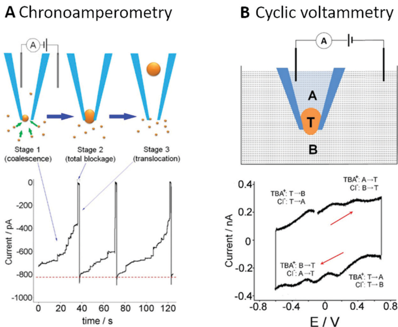
Fig. 26 Electrochemical sensing of single droplets by blocking: the ionic current of TBA + in water between two Ag/AgCl electrodes, one within the bulk phase, the other one confined within a quartz nanopipette with 200 nm orifice diameter is damped by the blockage of the orifice by adsorbed toluene + IL-PA droplets. (A) Amperometric current response of TBA + ionic current damped by adsorption and following droplet coalescence (stage 1). Complete blockage of the orifice exhibits a recorded current of 0 pA (stage 2), as the coalescent droplet translocates from the orifice into the pipette and the ionic current is fully restored (stage 3). (B) CV of ion transfer of TBA + and Cl - through a toluene + IL-PA coalescent nanodroplet, completely blocking the nanopipette orifice. Red lines indicate the scan direction. The recorded scan-rate is 20 V s -1 . Reproduced with permission from C. G. Gunderson, Z. Peng and B. Zhang, Langmuir , 2018, 34 , 2699. 174
