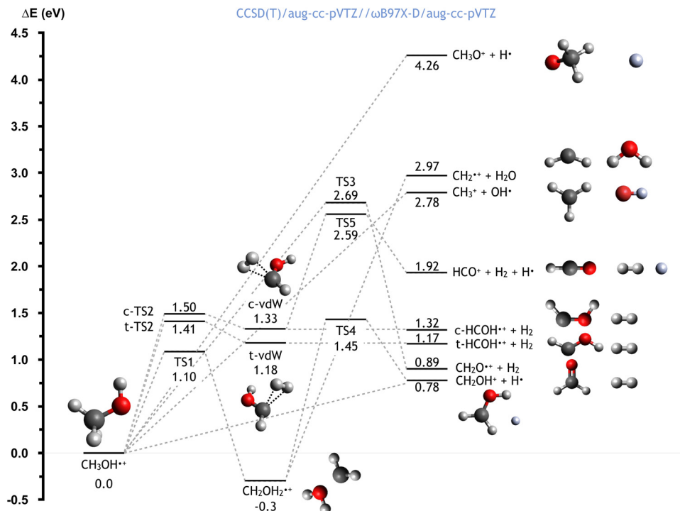
Fig. 6 Schematic representation of the PES for the dissociation of the CH 3 OH •+ cation, with the energies (reported in eV) evaluated at the CCSD(T)/aug-cc-pVTZ// \omega B97X-D/aug-cc-pVTZ level of theory. A similar figure with the energies computed at the CCSD(T)/aug-cc-pVTZ//B3LYP/aug-cc-pVTZ level is reported in the ESI.†
