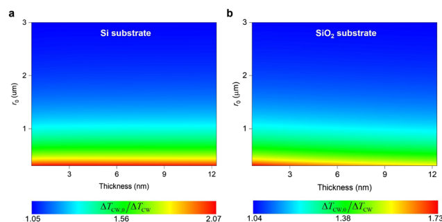
Fig. 11 Calculated temperature rise ratio of a supported \text{MoS}_2 film on (a) Si, and (b) a \text{SiO}_2 substrate.
