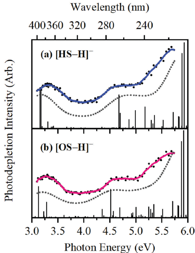
Fig. 4 Gas-phase experimental photodepletion spectra (solid colored line) vs. theoretical UV absorption spectra (dotted black line) calculated at the [\text{RI-MP2}/\text{ADC}(2)]/\text{aug-cc-pVDZ} level for (a) [\text{HS} - \text{H}]^- and (b) [\text{OS} - \text{H}]^- , respectively; theoretical UV absorption spectra were phenomenologically broadened with Lorentzian functions (FWHM = 0.8 eV). The vertical lines represent the calculated vertical excitation energies.
