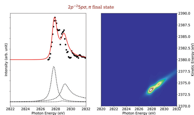
Fig. 8 Cross section of the 2p^{-2}5p\sigma, \pi (left) as a function of the photon energy, the black dots are the experimental points and the solid line is the result of our simulation. The dashed lines in the lower part of the figure display the contributions of the individual intermediate states. The simulated contributions of this final state to the 2D-map are displayed on the right-hand side of the figure.
